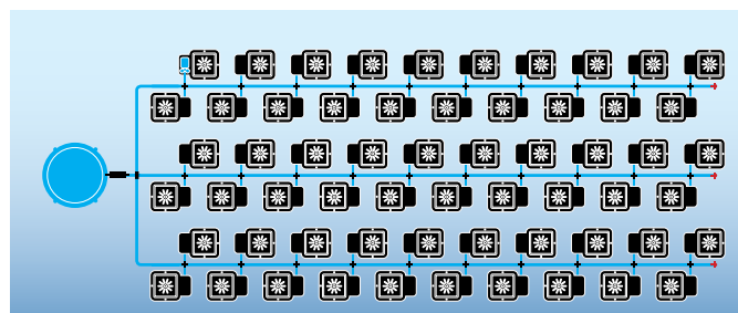
Complete 60 Pot System with 750L FlexiTank
